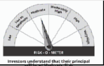
Benchmark Risk-O-Meter
