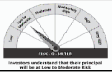
Scheme Risk-O-Meter
